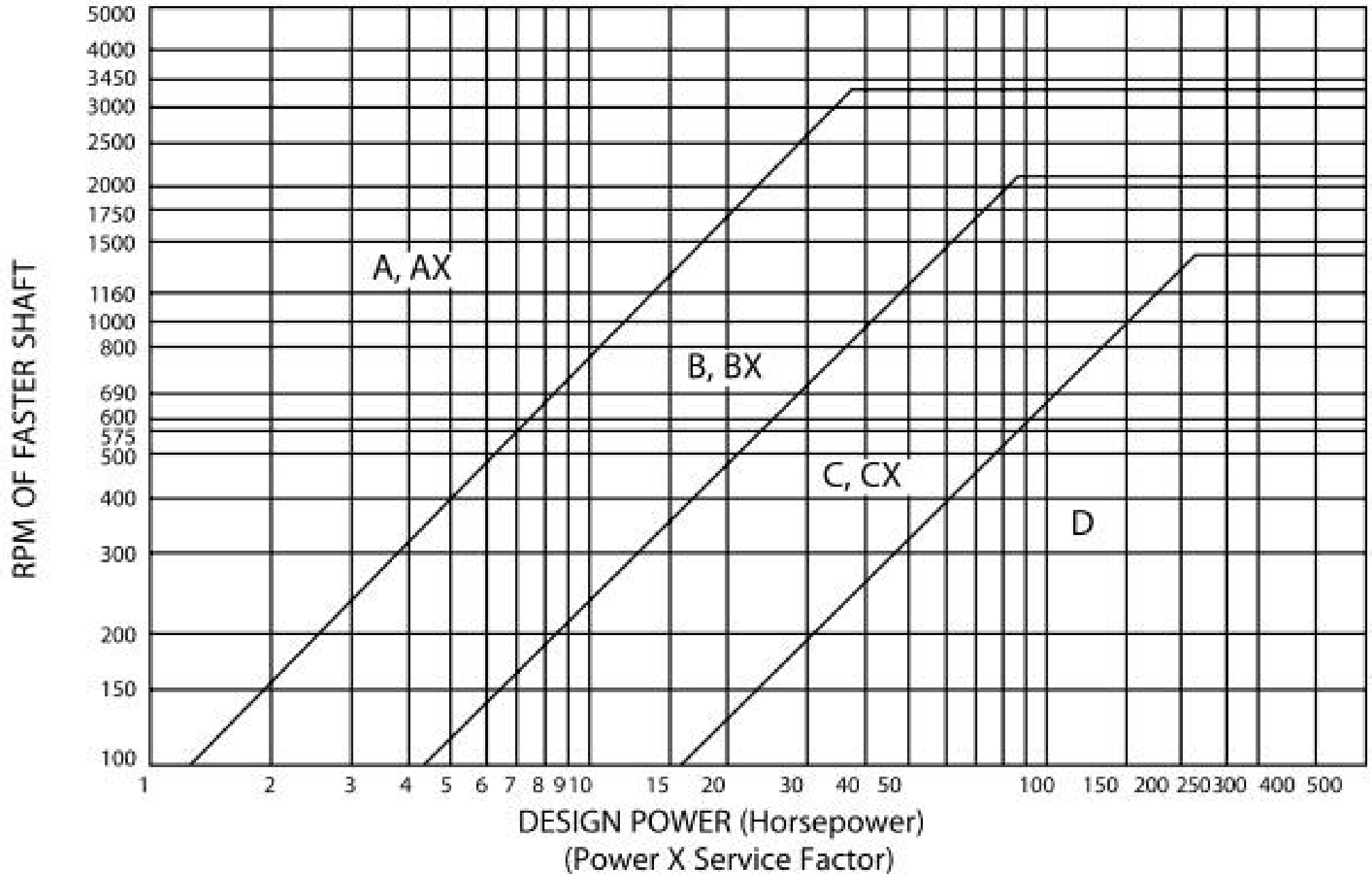
FIGURE 1: CLASSICAL V-BELTS
