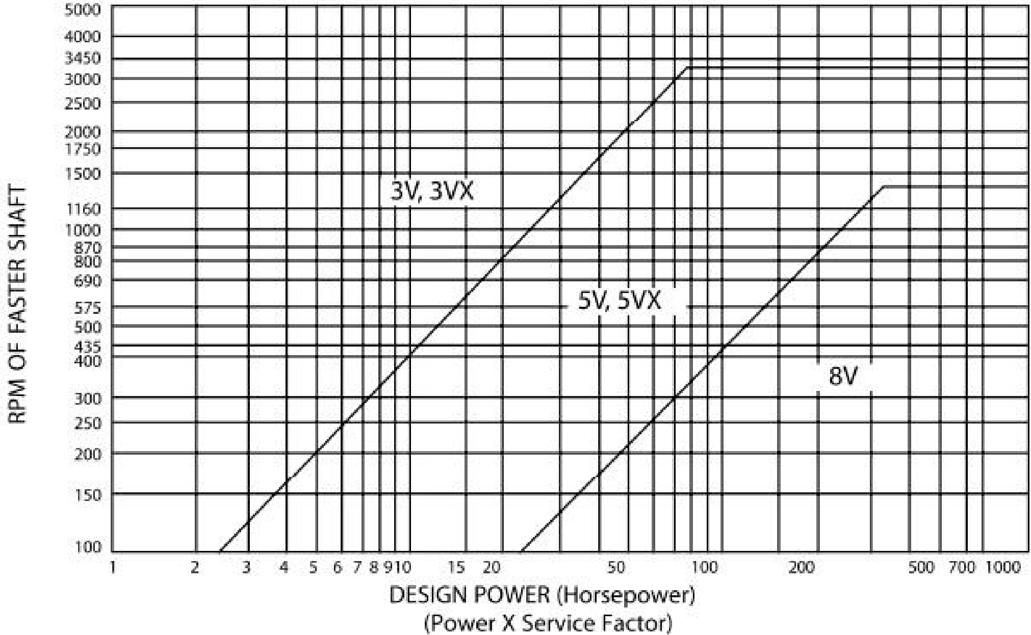
FIGURE 2: NARROW V-BELTS
